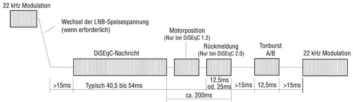
DiSEqC 1.0 Sequenz
